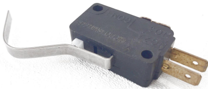
SWITCH WITH BENT ARM Part Number: C08258.0000
